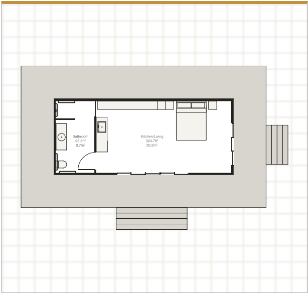
Plan B, deck along the front
