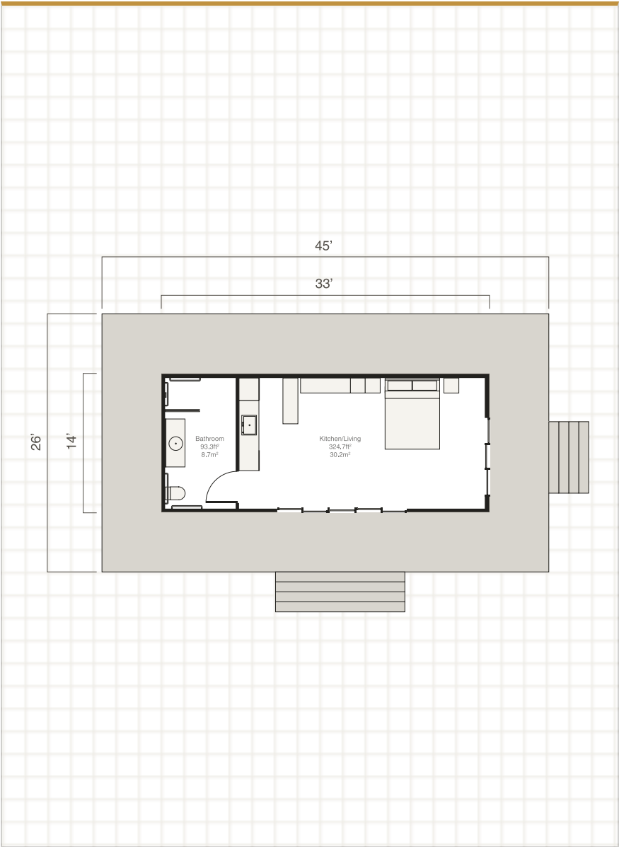
Floor plan with a 45 × 26 ft deck. Plans B and C place the deck on the long side instead.
