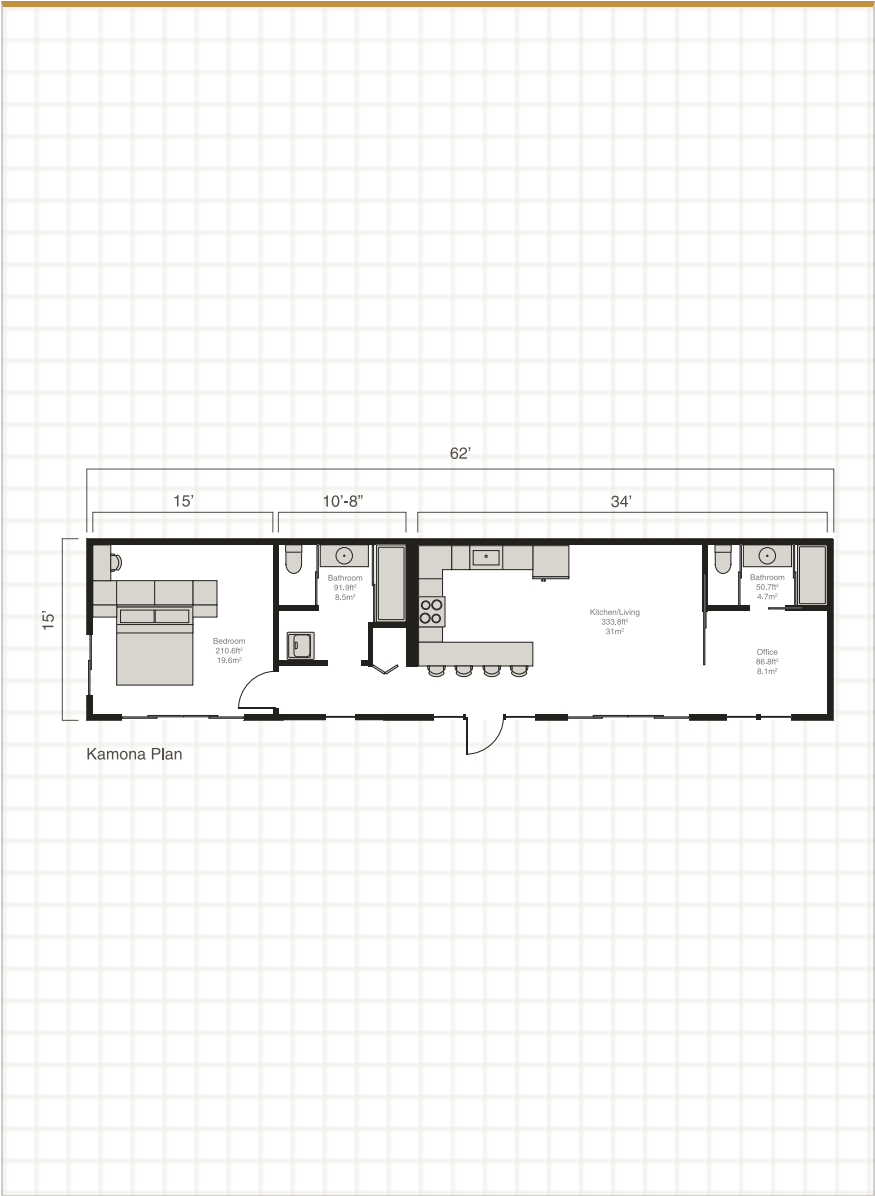
Floor plan, 62 × 15 ft: bedroom, bathroom, office, kitchen and living room, second bathroom.
